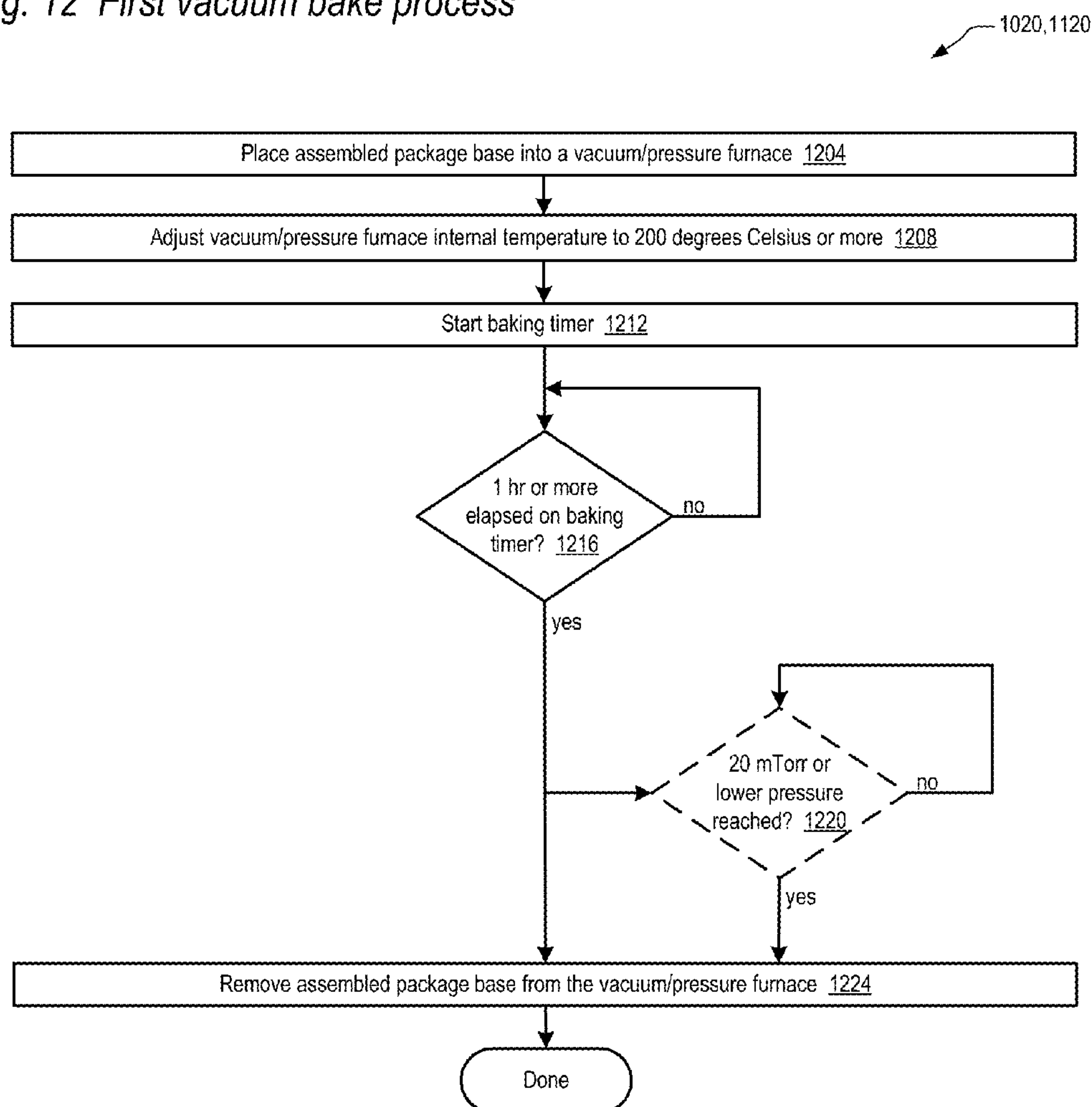
Fig. 12 First vacuum bake process
