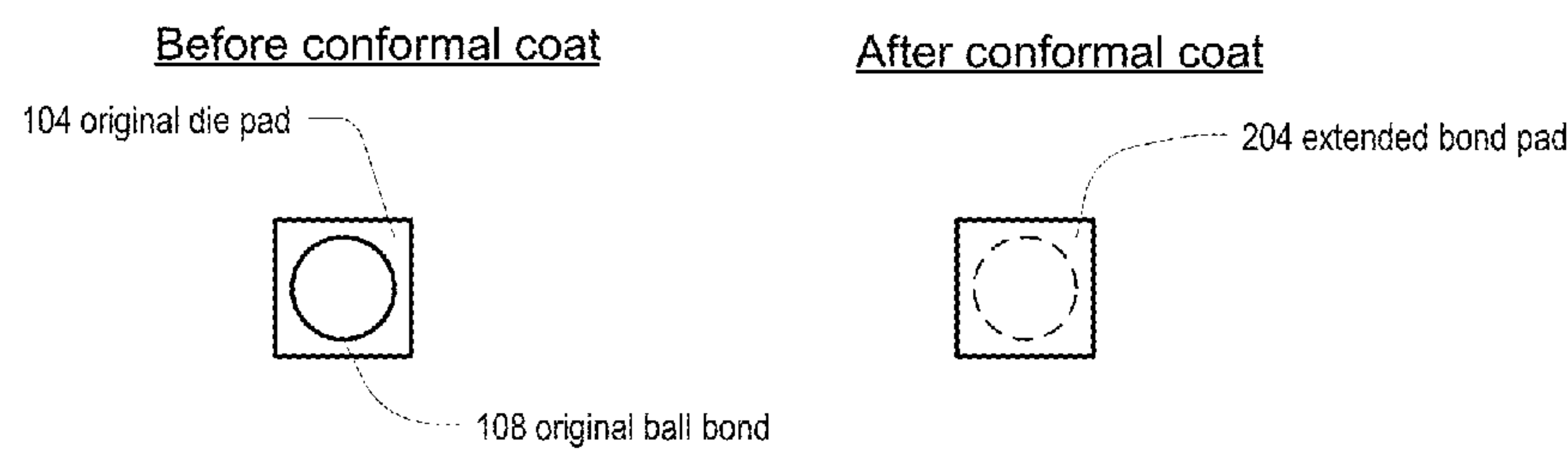
Fig. 2a Extended bond pad first geometry
