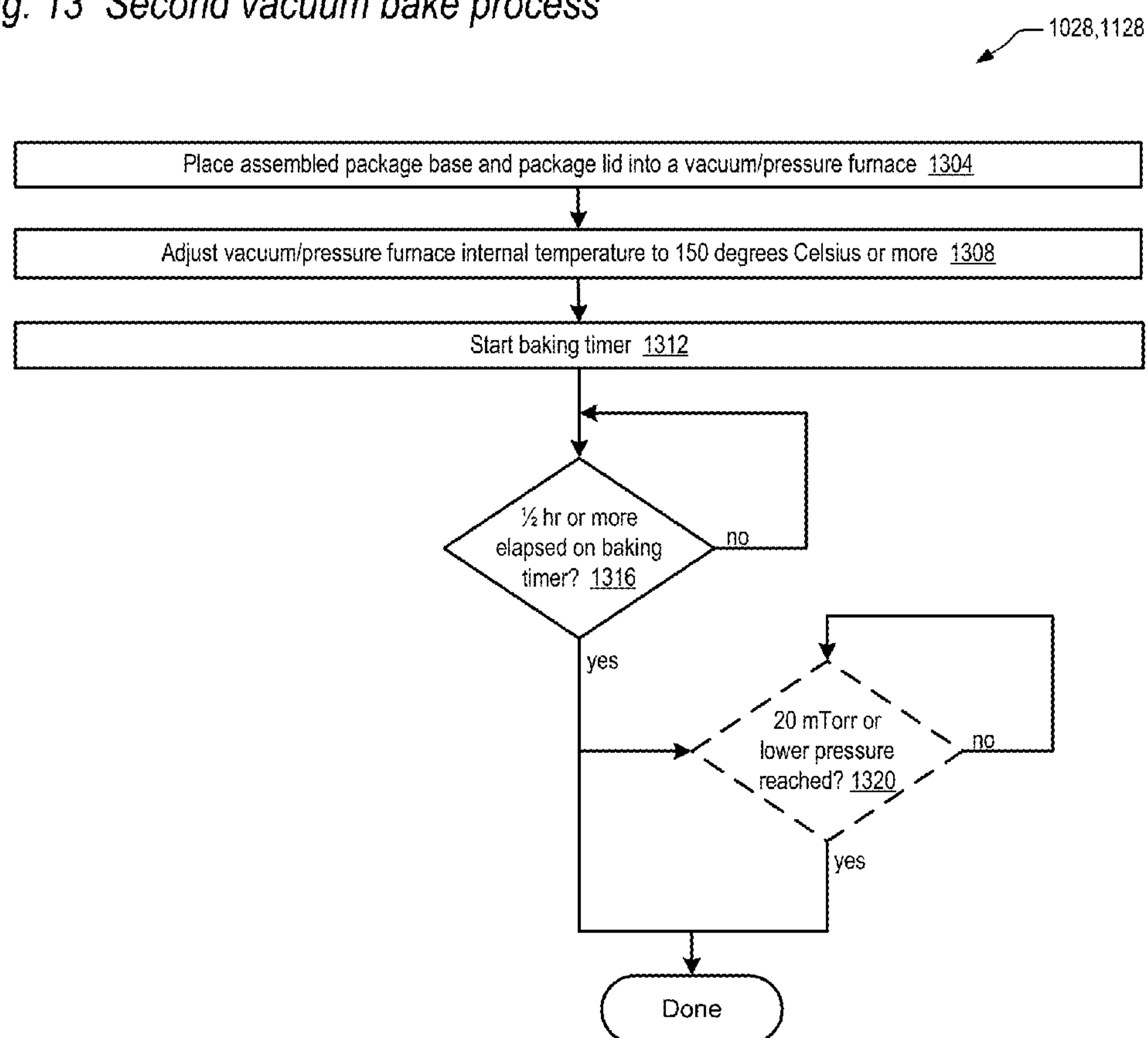
Fig. 13 Second vacuum bake process
